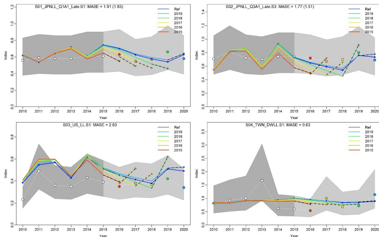
Figure 18. Hind casting cross-validation (HCxval) results for the four CPUE fits, showing observed (large points with dashed line), fitted (solid lines), and one-year-ahead forecast values (small terminal points) in the old growth model. The observations used for cross-validation are highlighted as color-coded solid circles with associated 95% confidence intervals (light-grey shading). The model reference year refers to the endpoint of each one-year-ahead forecast and the corresponding observation. The mean absolute scaled error (MASE) score associated with each CPUE time series is denoted in each panel.
