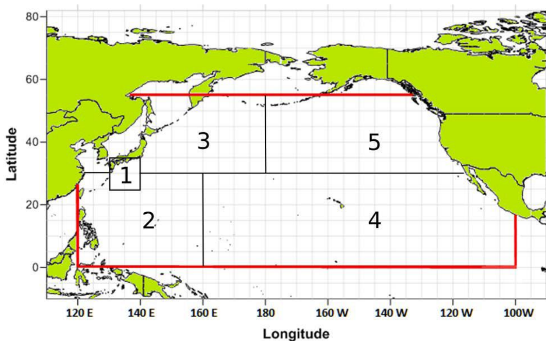
Figure 4. Spatial domain (red box) of the north Pacific albacore stock ( Thunnus alalunga ) in the 2017 stock assessment. Fishery definitions were based on five fishing areas (black boxes and numbers) defined from cluster analyses of size composition data.
