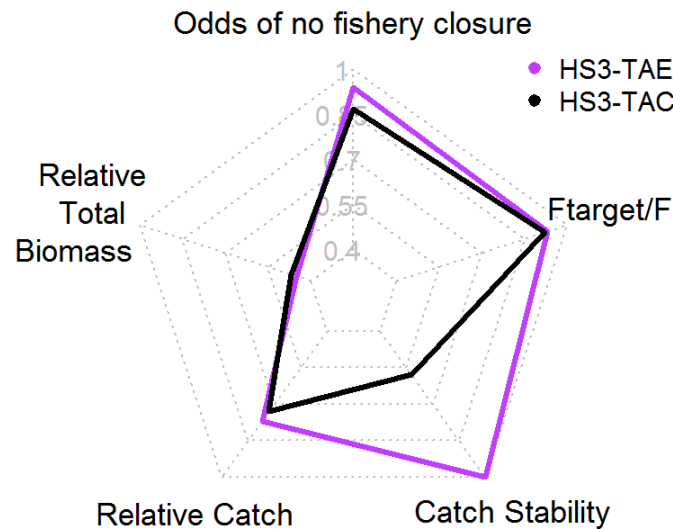
Figure ES8. Cobweb plot depicting performance indicators for TAC-based and TAE-based HCR13 for HS3 for all runs and reference scenarios. Values close to the outer web signify a more positive outcome for that performance indicator. Relative catch is defined as the odds of catch in any given year of the MSE forward simulation being above average historical (1981-2010) catch. Relative total biomass is defined as the odds of depletion in any given year of the MSE forward simulation being above minimum historical (2006-2015) depletion. Odds of no fishery closure is the probability that SSB in any given year of the MSE forward simulation is above the LRP. Catch stability is defined as the probability that a decrease in TAC is <30% between consecutive assessment periods (once every 3 years), excluding years where TAC=0. Ftarget/F is the ratio of the F specified by the TRP to the actual fishing intensity in the operating model (OM).
