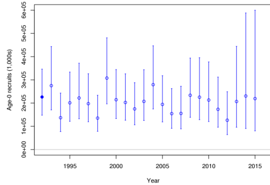
Figure 7-1. Maximum likelihood estimates of (A) total age-1+ biomass (open circles) (B), female spawning biomass (SSB) (solid blue line), and (C) age-0 recruitment (open circles) of north Pacific albacore tuna ( Thunnus alalunga ). Dashed lines (B) and vertical bars (C) indicate 95% confidence intervals of the female SSB and recruitment estimates respectively. Red line indicates the 20%SSB current, F=0 limit reference point, which is based on dynamic SSB 0 . Closed black circle and error bars in (B) are the maximum likelihood estimate and 95% confidence intervals of unfished female spawning biomass, SSB 0 . Since the assessment model represents time on a quarterly basis, there are four estimates of total biomass (A) for each year, but only one annual estimate of female SSB (B) and recruitment (C).
