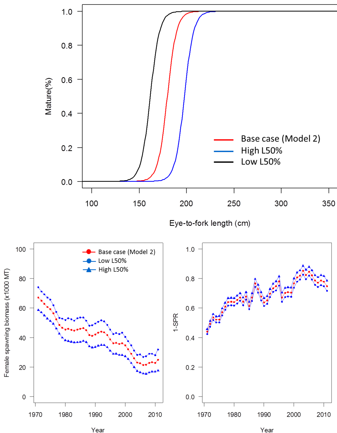
Figure 9.9.5. Results of size at 50% maturity sensitivity analysis for the base case Stock Synthesis model.
