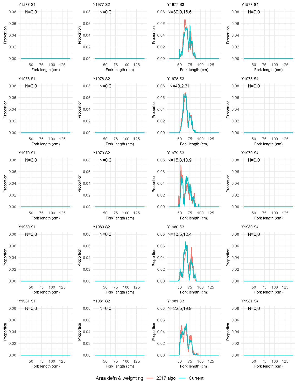
Figure 1. Seasonal size compositions (red: 2017 algorithm; blue: current algorithm) for the U.S. surface fishery for 1977 – 2018. N indicate the input sample size for size compositions.
